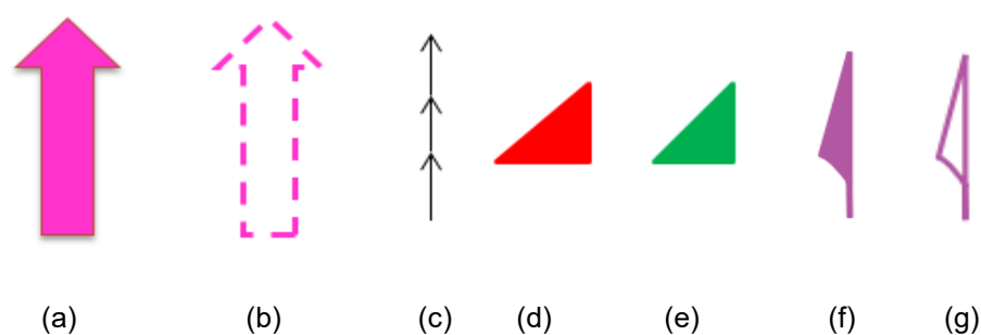
Figure 9-2 – Existing arrow types and approximate colours approved for use in ECDIS: (a) and (b) for Traffic Separation Schemes; (c) for recommended (one-way) tracks; (d) and (e) for conical buoys; and (f) and (g) for magnetic variation and anomaly
