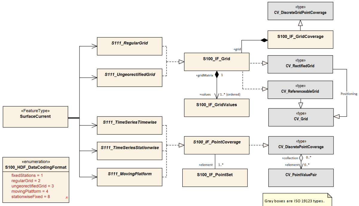
Figure 4-3 – Coverages and their realisation from S-100 Part 8 and ISO 19123
