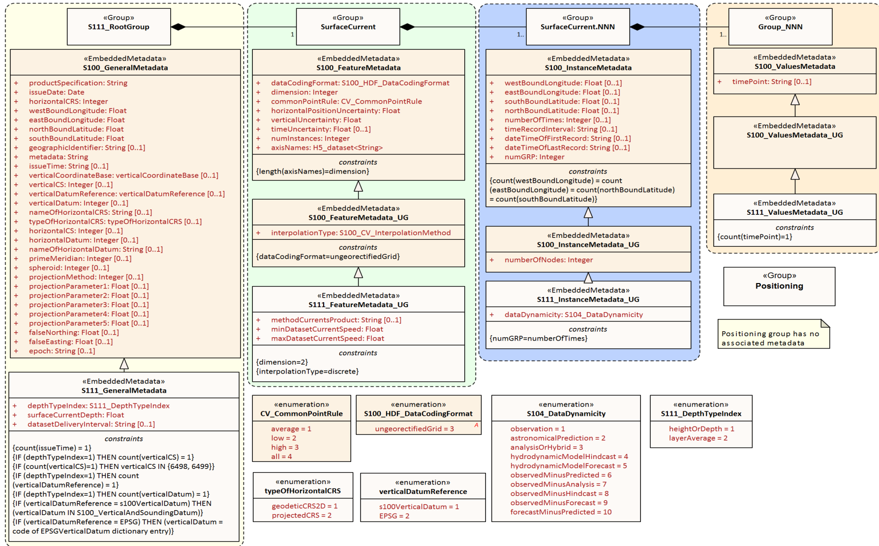
Figure B-8 – All carrier metadata for coverage type Ungeorectified Grid (data coding format 3)
