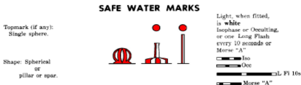
Figure 20-8 – IALA safe water beacons – Characteristics
