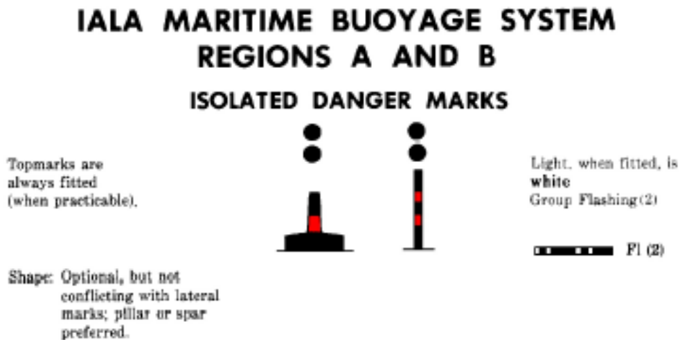
Figure 20-3 – IALA isolated danger buoys – Characteristics
