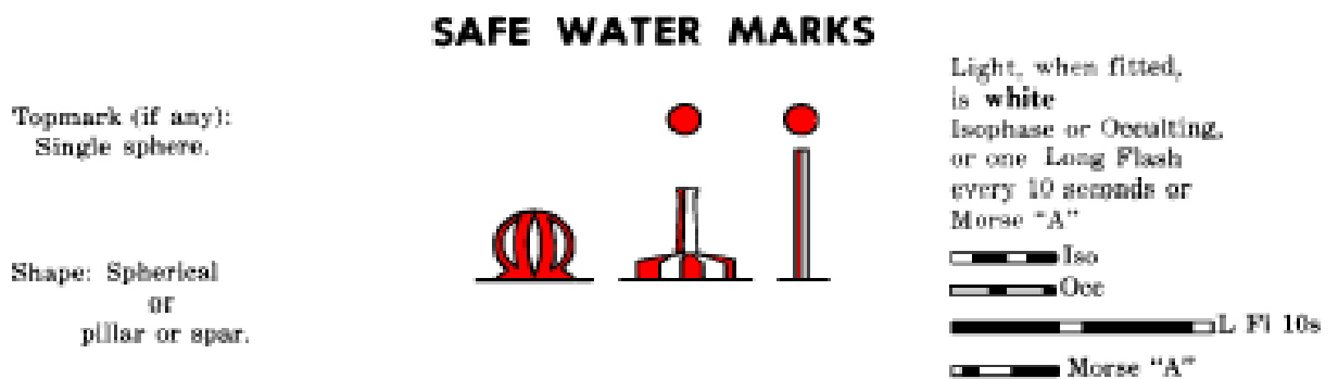
Figure 20-4 – IALA safe water buoys – Characteristics
