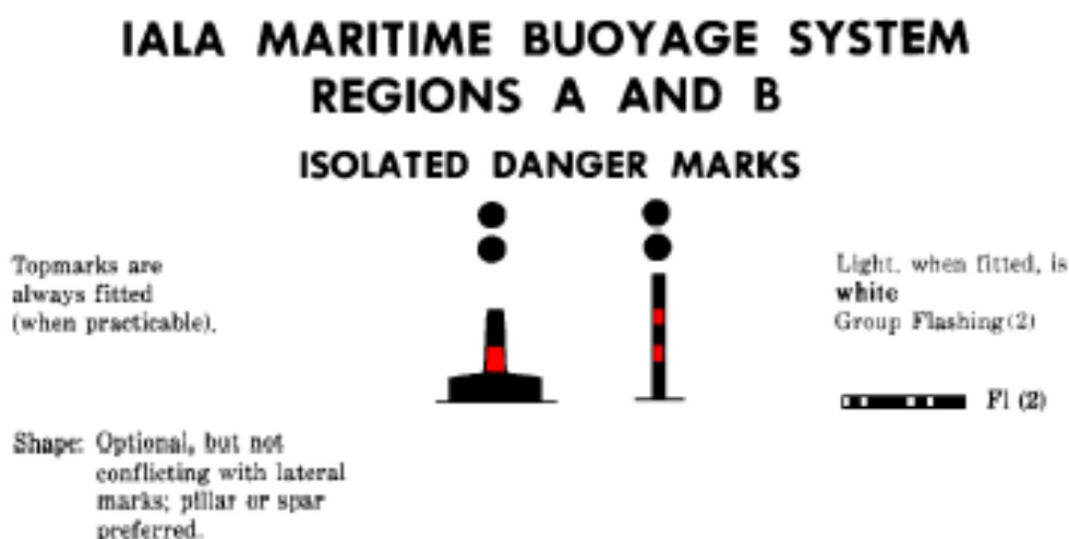
Figure 20-7 – IALA isolated danger beacons – Characteristics
