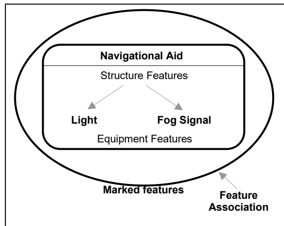
Figure 18-1 – Navigational aids – Structure/equipment association
