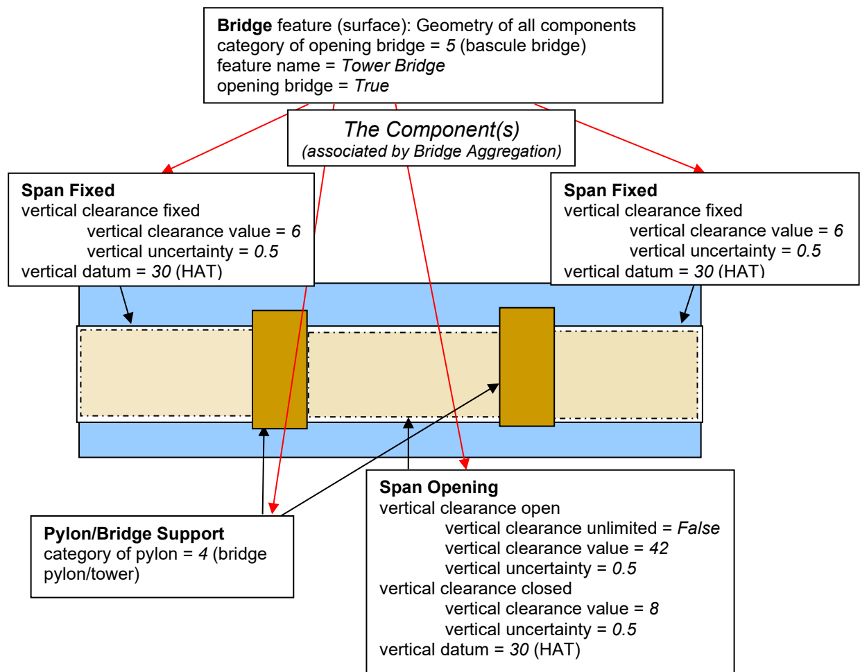
Figure 6-2 – Bascule bridge – Example
